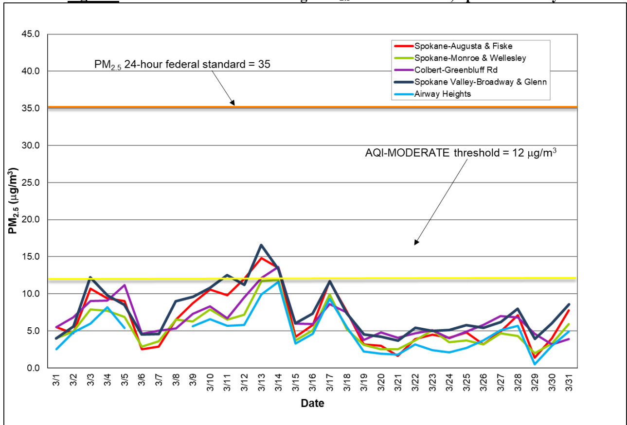
Figure 2: Multi-station 24-hour average PM 2.5 for March 2021; Spokane County.
