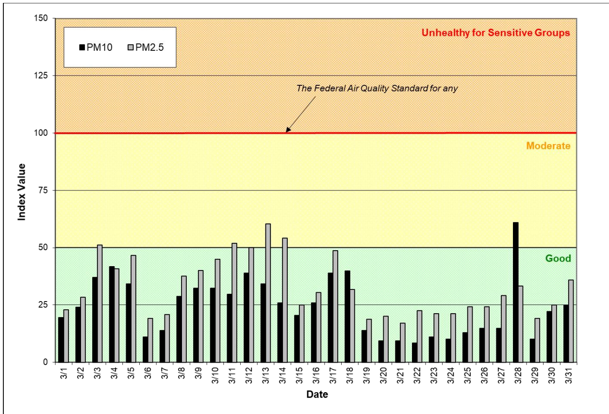
Figure 1: Air Quality Index (AQI) values for March 2021. The data represent the maximum AQI values across all monitoring stations within Spokane County.
