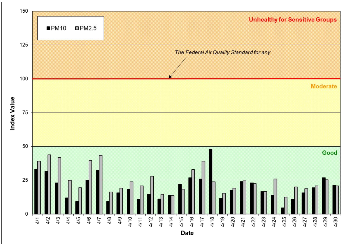
Figure 1: Air Quality Index (AQI) values for April 2021. The data represent the maximum AQI values across all monitoring stations within Spokane County.
