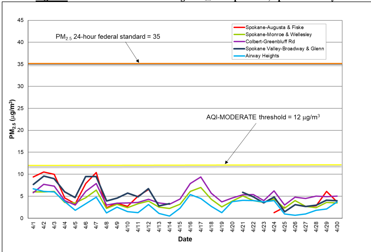
Figure 2: Multi-station 24-hour average PM 2.5 for April 2021; Spokane County.
