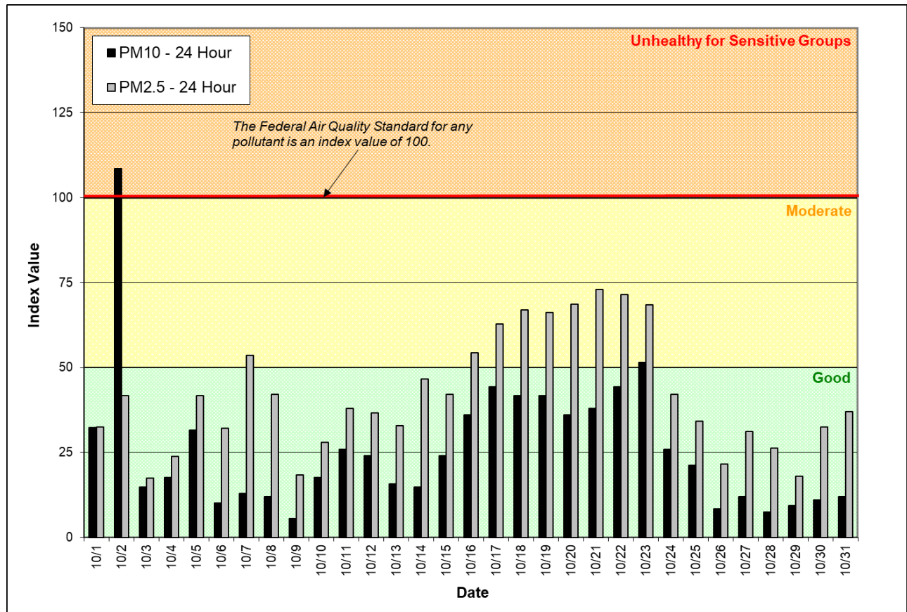
Figure 1: Air Quality Index (AQI) values for October 2018. The data represent the maximum AQI values across all monitoring stations within Spokane County.
