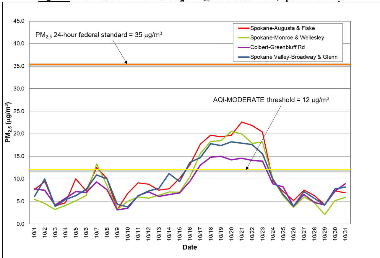
Figure 2: Multi-station 24-hour average PM_{2.5} for October 2018; Spokane County.
