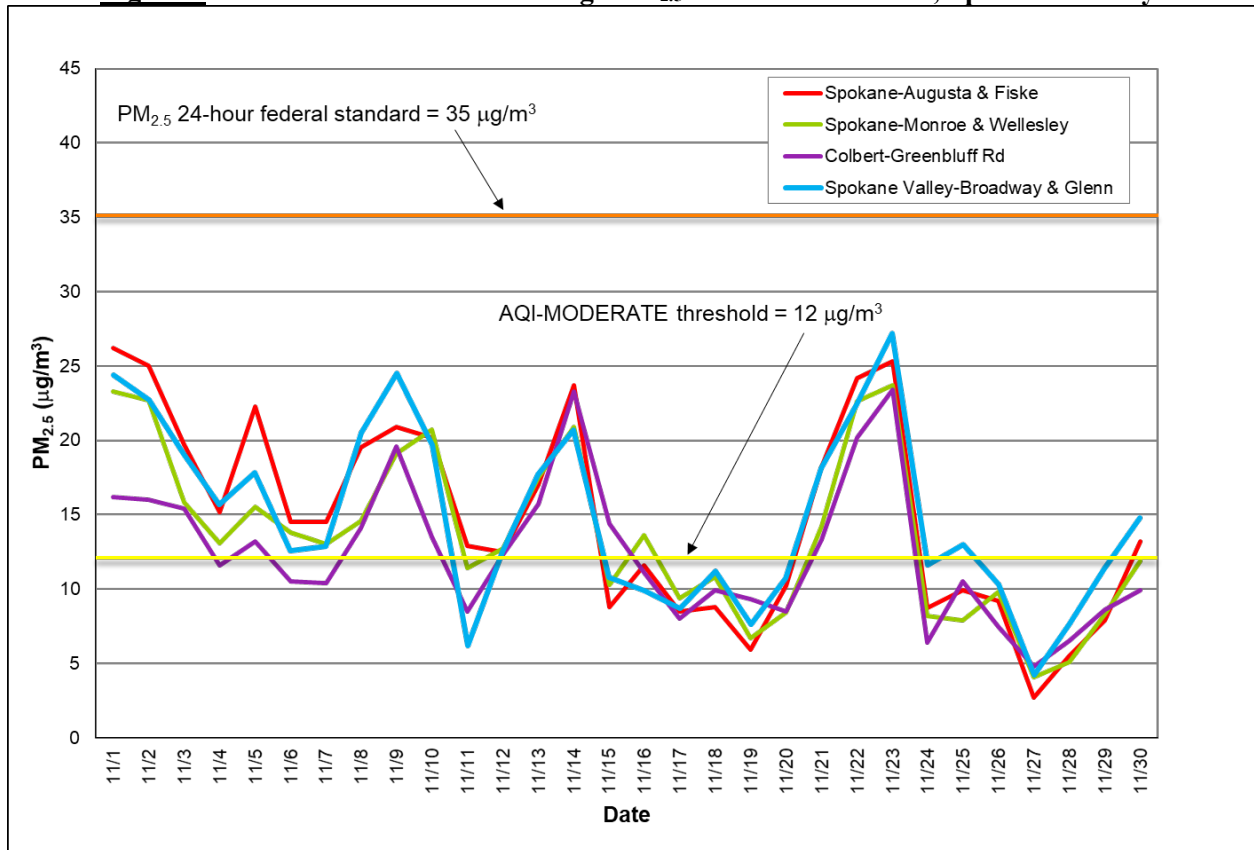
Figure 2: Multi-station 24-hour average PM 2.5 for November 2019; Spokane County.
