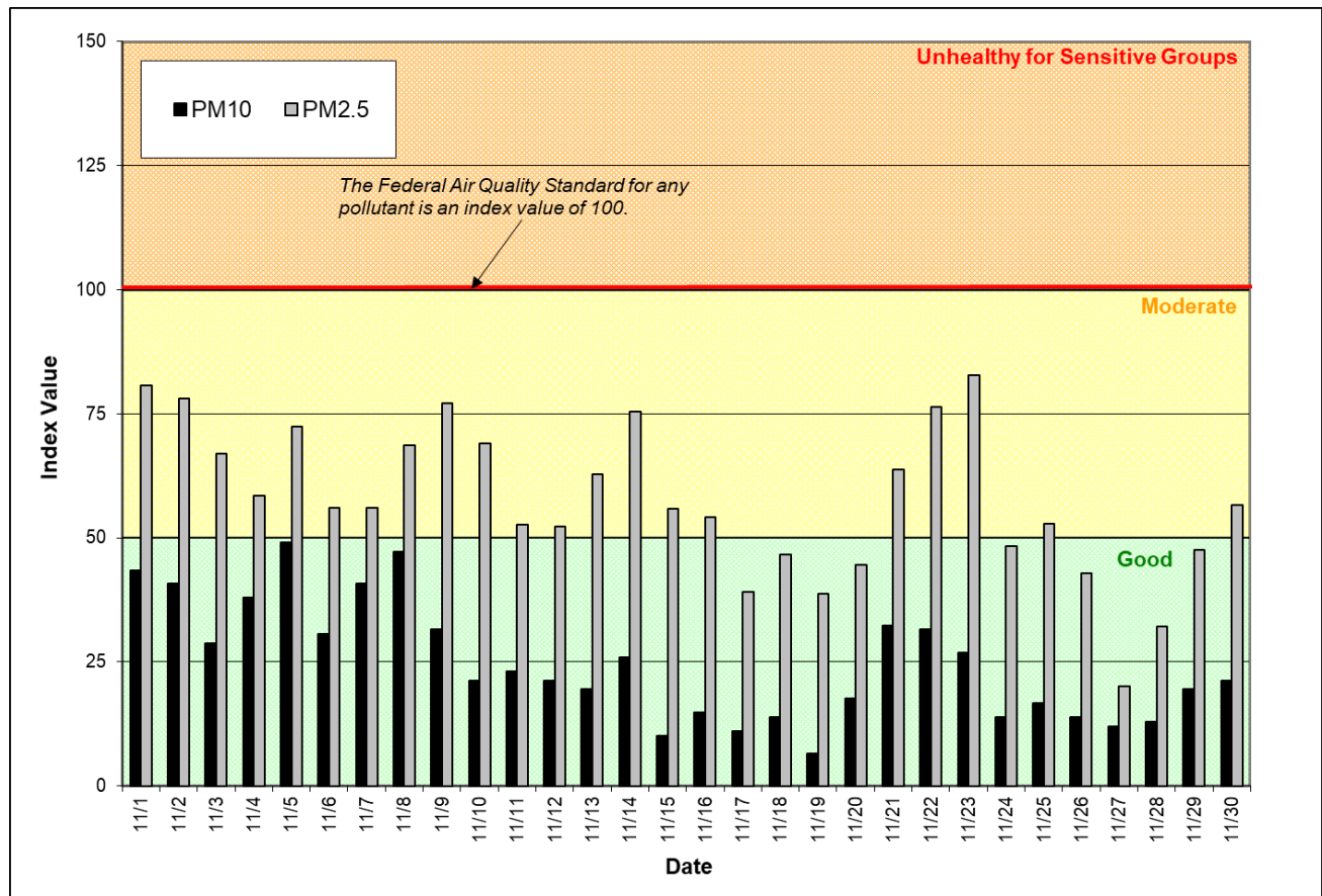
Figure 1: Air Quality Index (AQI) values for November 2019. The data represent the maximum AQI values across all monitoring stations within Spokane County.
