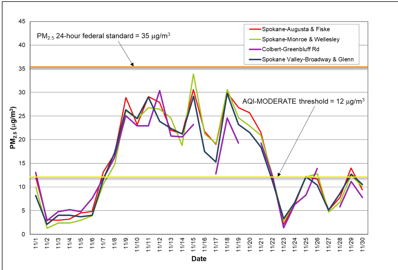
Figure 2: Multi-station 24-hour average PM 2.5 for November 2018; Spokane County. Loss of PM 2.5 data from the Colbert monitoring station occurred because of instrument enclosure HVAC problems on the 16 th and 20 th and downtime for work to modify the station's electrical circuit on the 27 th .
