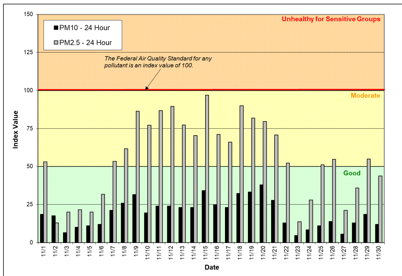
Figure 1: Air Quality Index (AQI) values for November 2018. The data represent the maximum AQI values across all monitoring stations within Spokane County.
