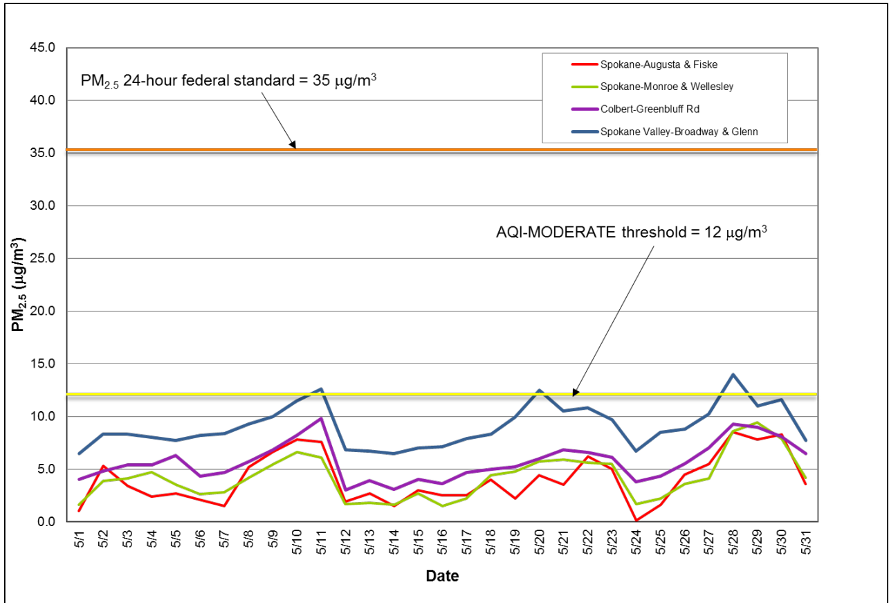
Figure 2: Multi-station 24-hour average PM 2.5 for May 2017; Spokane County.
