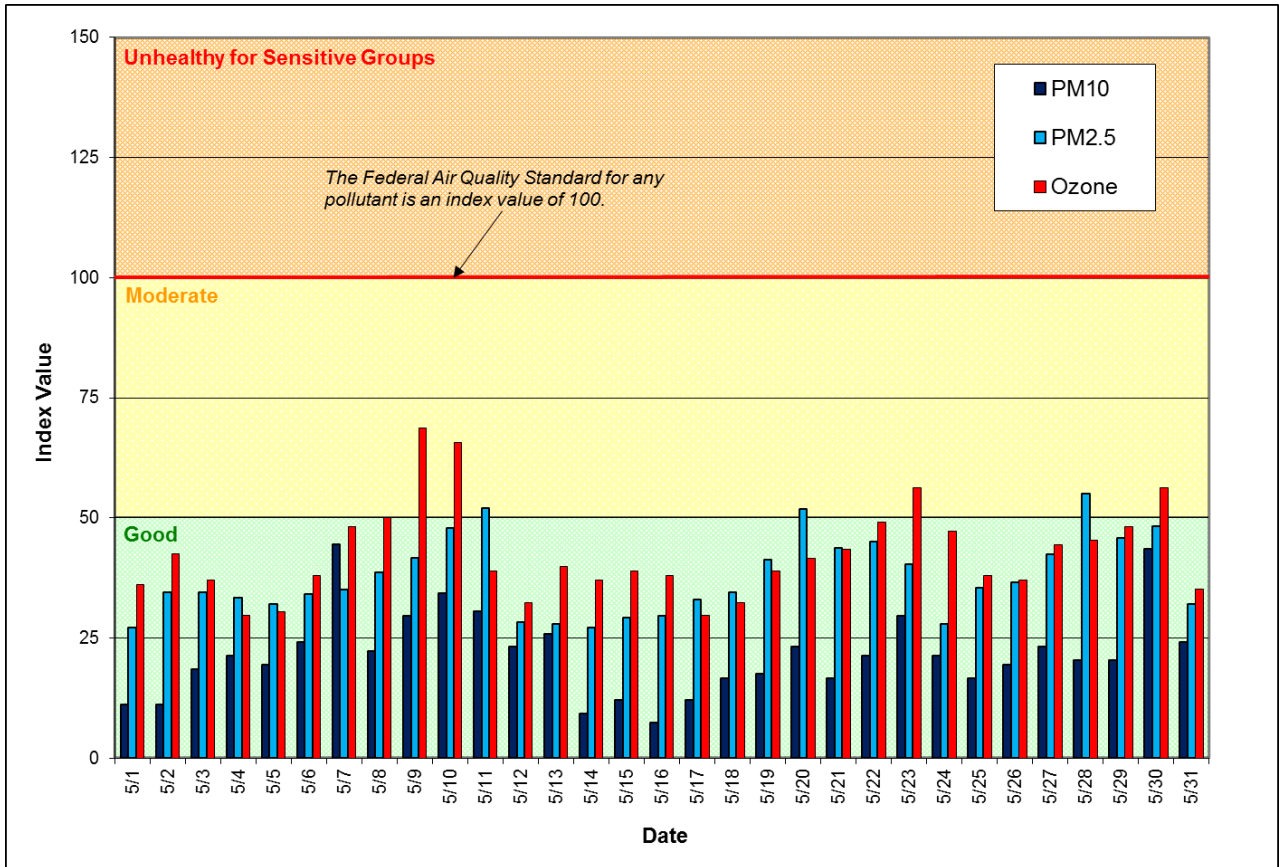
Figure 1: Air Quality Index (AQI) values for May 2017. The data represent the maximum AQI values across all monitoring stations within Spokane County.
