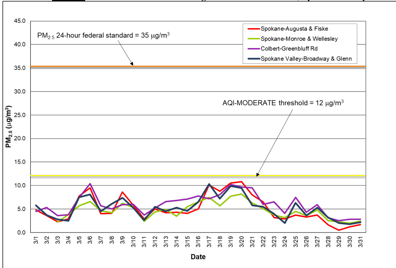
Figure 2: Multi-station 24-hour average PM 2.5 for March 2020; Spokane County.
