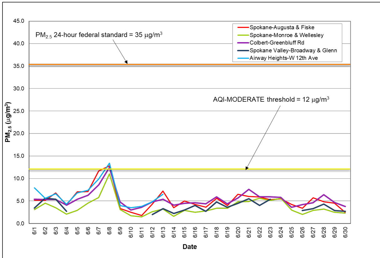
Figure 2: Multi-station 24-hour average PM 2.5 for June 2018; Spokane County.
