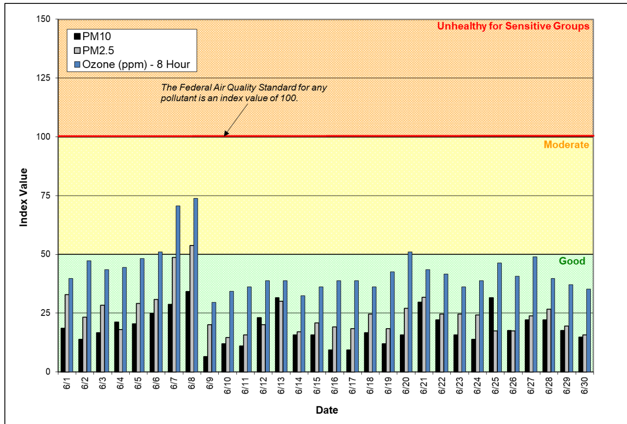
Figure 1: Air Quality Index (AQI) values for June 2018. The data represent the maximum AQI values across all monitoring stations within Spokane County.
