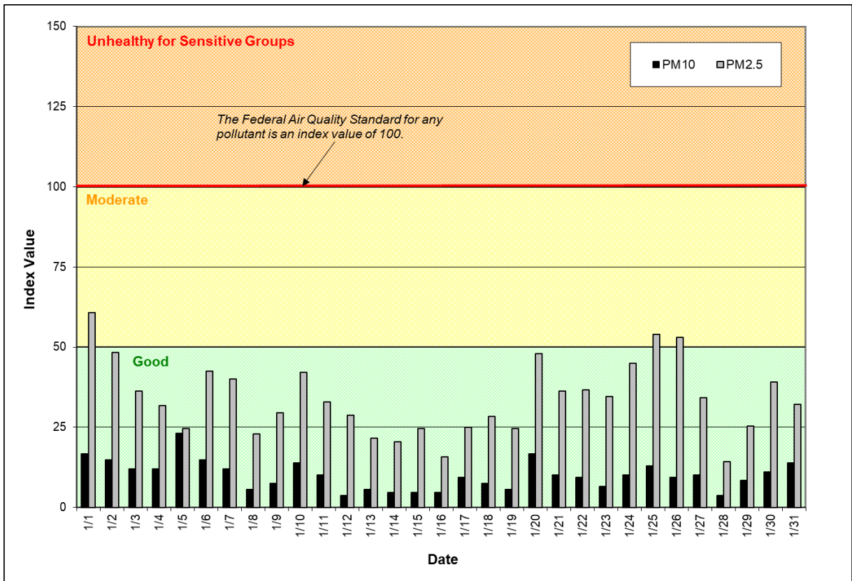
Figure 1: Air Quality Index (AQI) values for January 2023. The data represent the maximum AQI values across all monitoring stations within Spokane County.
