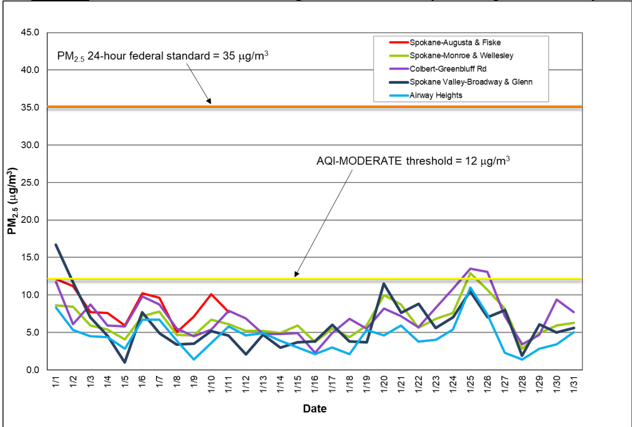
Figure 2: Multi-station 24-hour average PM 2.5 for January 2023; Spokane County.
