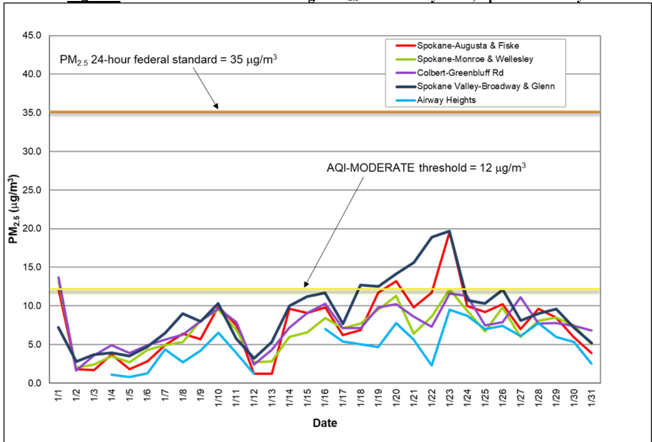
Figure 2: Multi-station 24-hour average PM 2.5 for January 2021; Spokane County.
