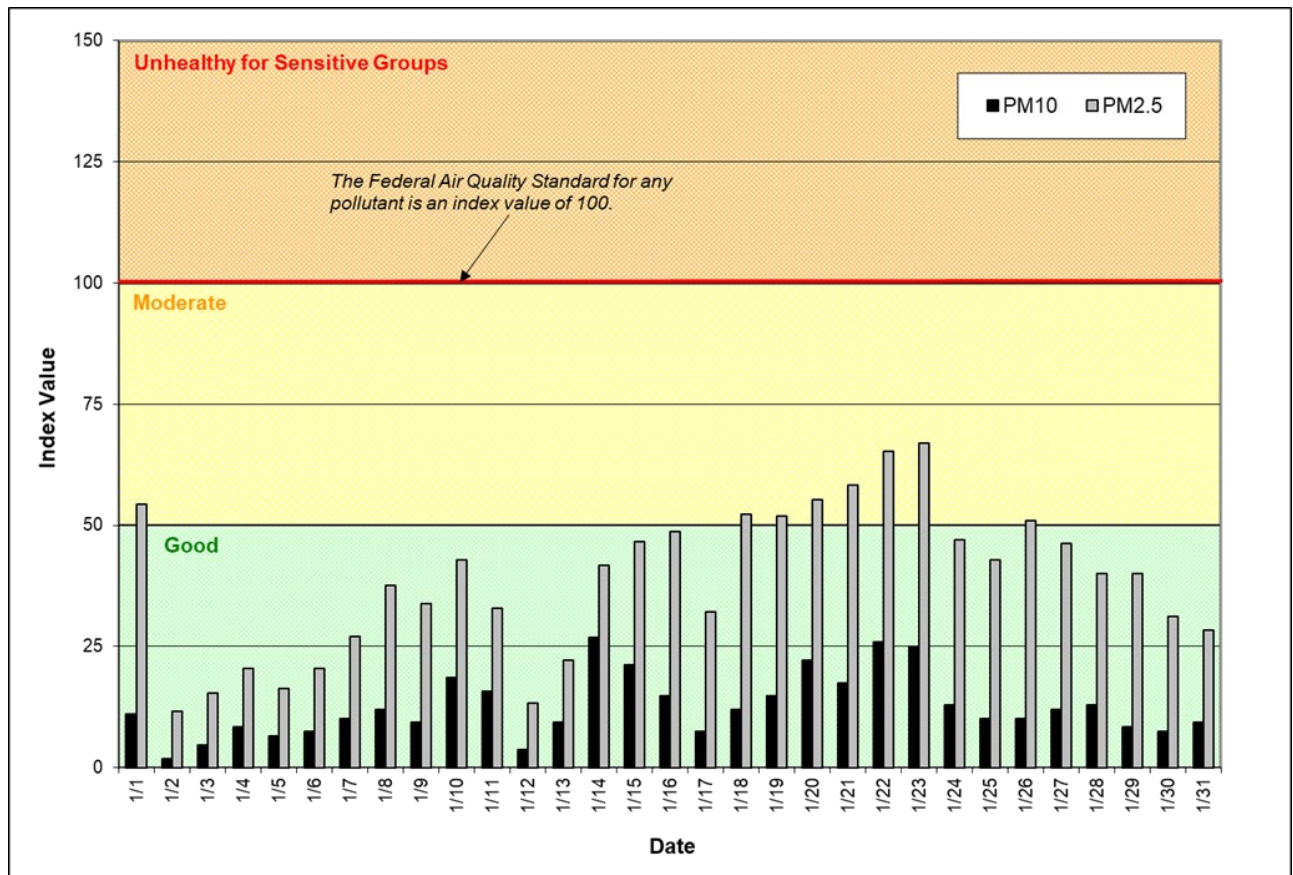
Figure 1: Air Quality Index (AQI) values for January 2021. The data represent the maximum AQI values across all monitoring stations within Spokane County.
