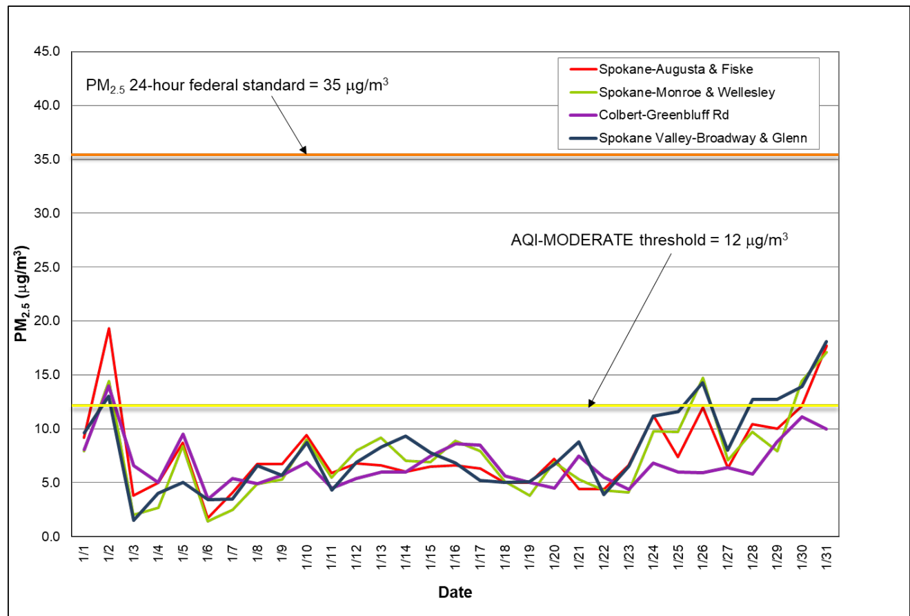
Figure 2: Multi-station 24-hour average PM_{2.5} for January 2019; Spokane County.
