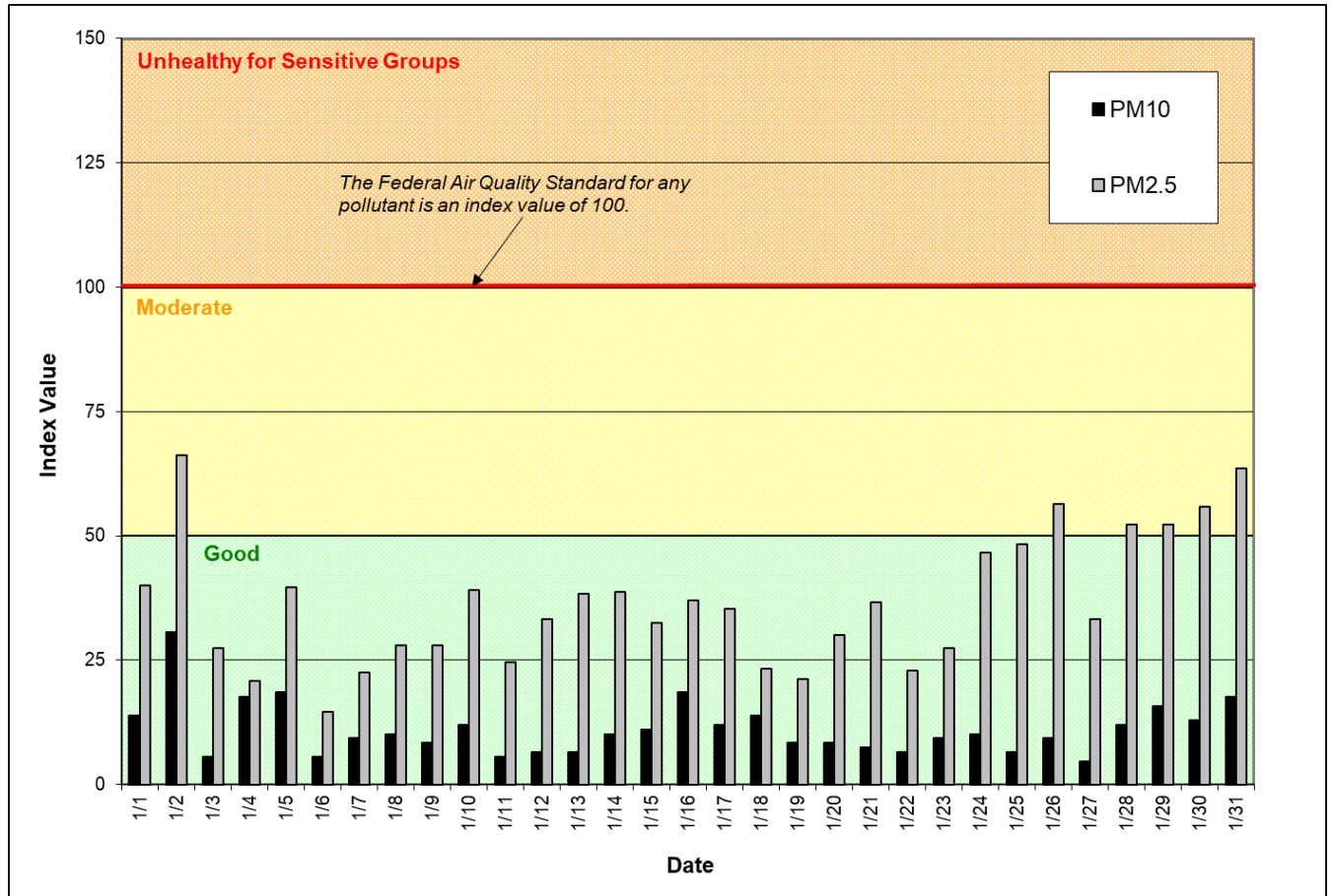
Figure 1: Air Quality Index (AQI) values for January 2019. The data represent the maximum AQI values across all monitoring stations within Spokane County.
