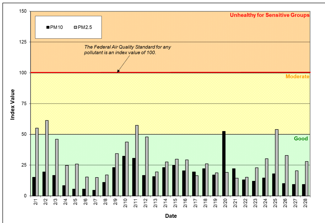
Figure 1: Air Quality Index (AQI) values for February 2023. The data represent the maximum AQI values across all monitoring stations within Spokane County.
