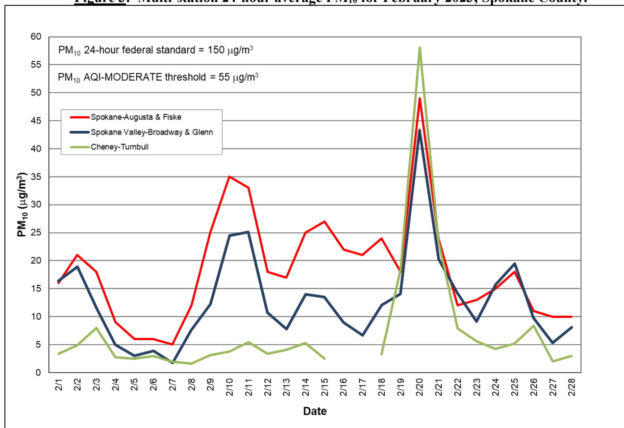
Figure 3: Multi-station 24-hour average PM 10 for February 2023; Spokane County.
