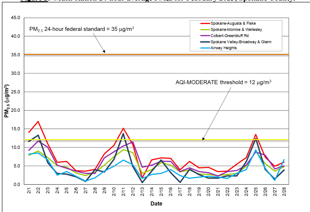
Figure 2: Multi-station 24-hour average PM 2.5 for February 2023; Spokane County.
