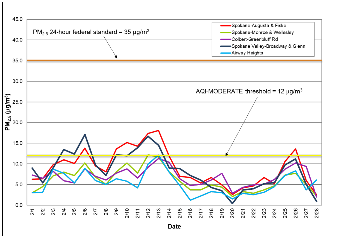
Figure 2: Multi-station 24-hour average PM 2.5 for February 2022; Spokane County.
