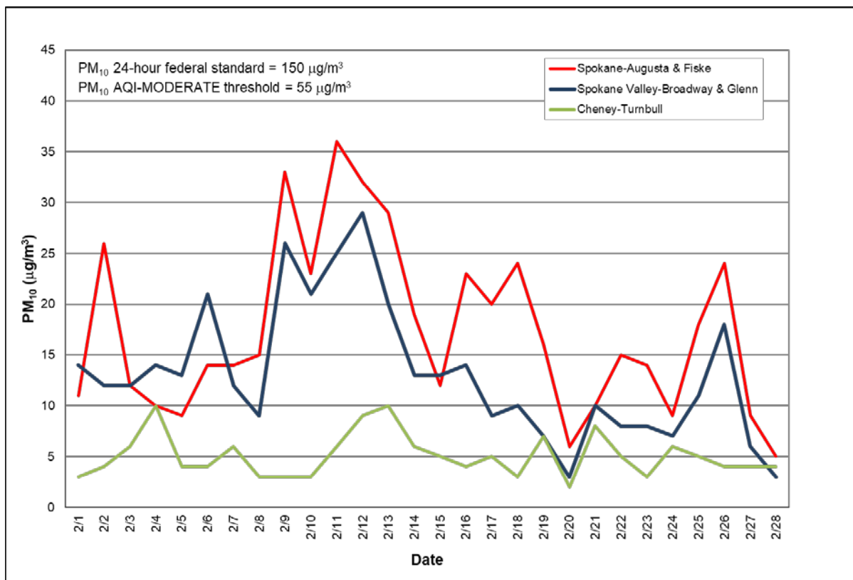
Figure 3: Multi-station 24-hour average PM 10 for February 2022; Spokane County.
