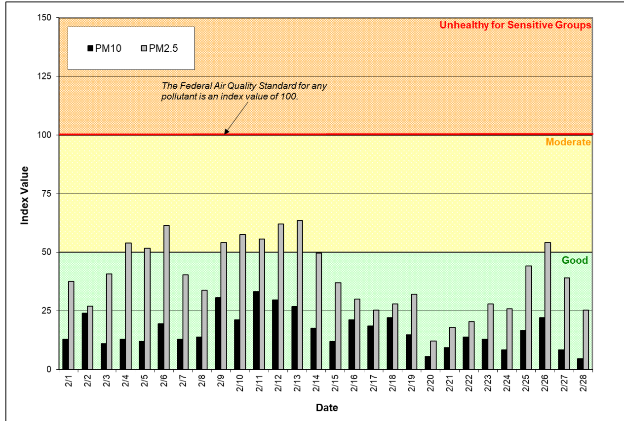
Figure 1: Air Quality Index (AQI) values for February 2022. The data represent the maximum AQI values across all monitoring stations within Spokane County.
