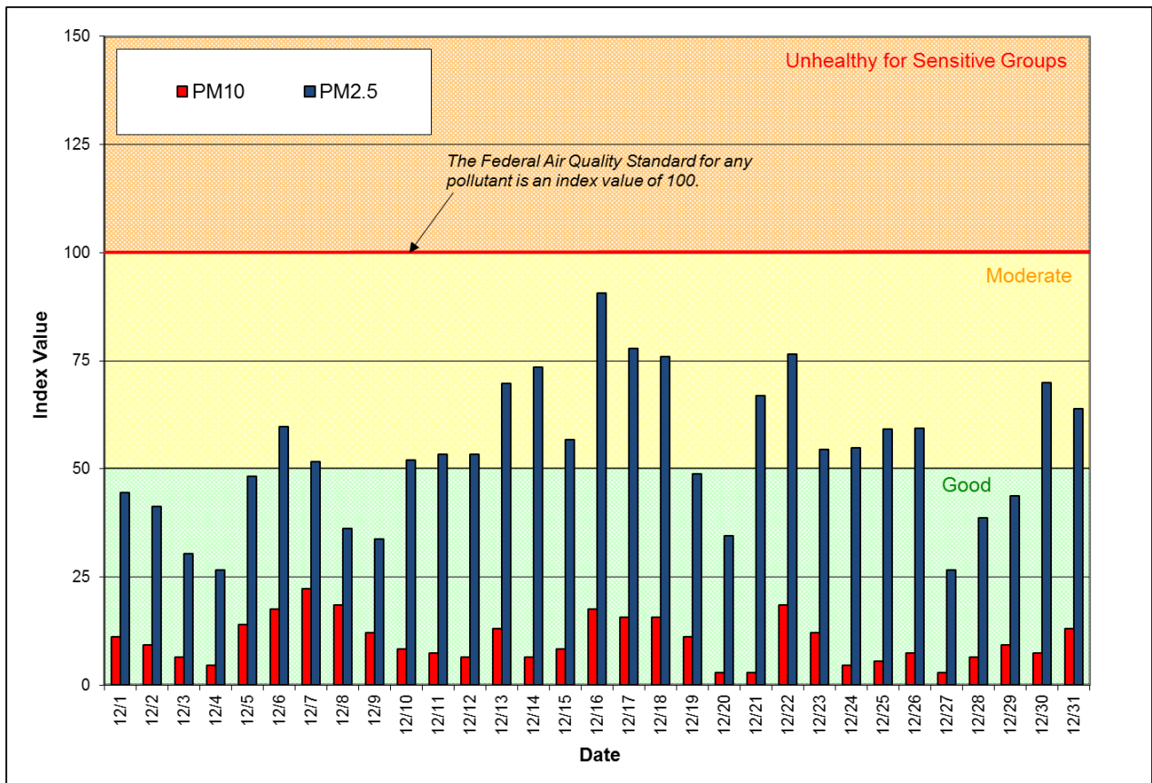
Figure 1: Air Quality Index (AQI) values for December 2016. The data represent the maximum AQI values across all monitoring stations within Spokane County.
