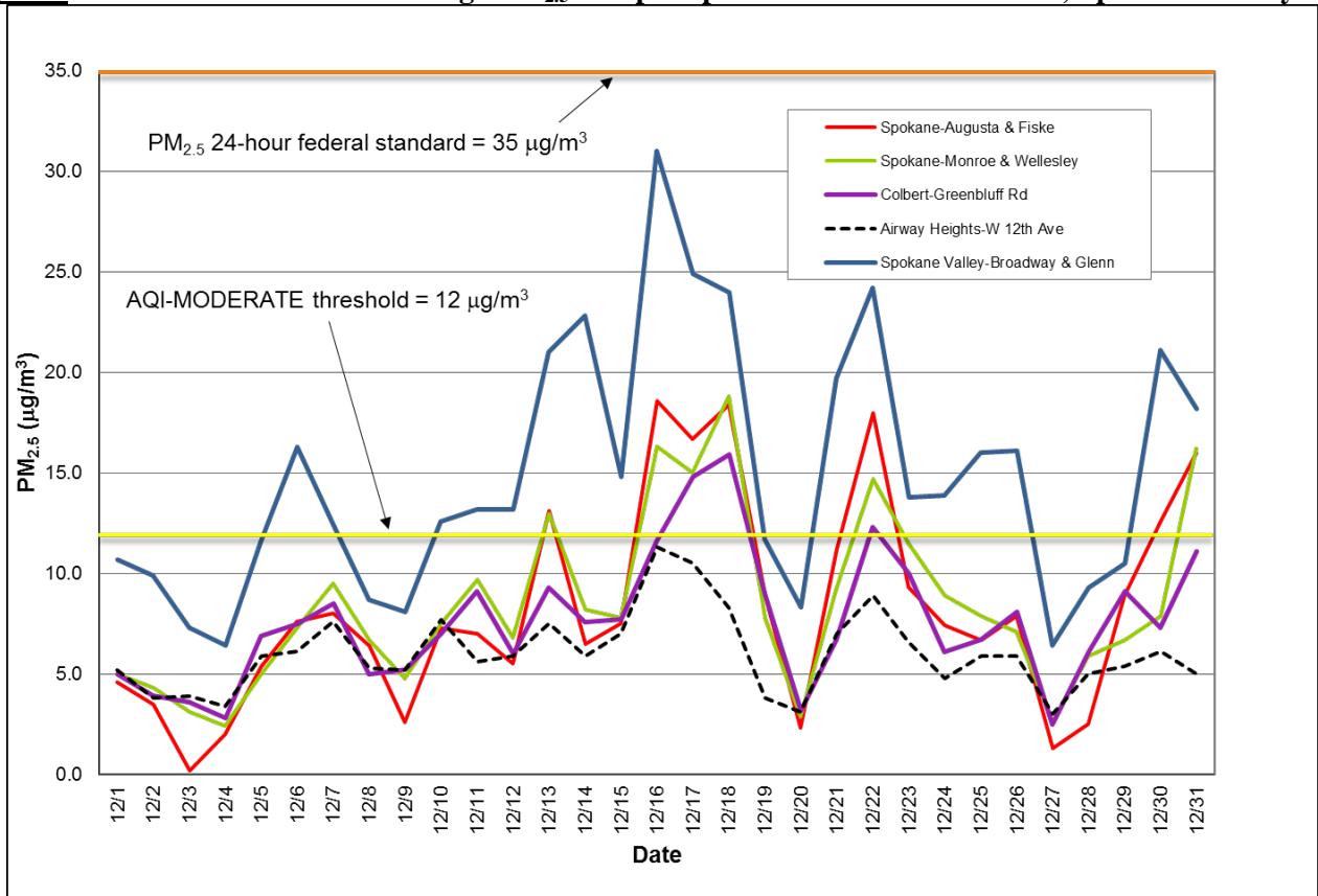
Figure 2: Multi-station 24-hour average PM 2.5 and precipitation for December 2016; Spokane County.
