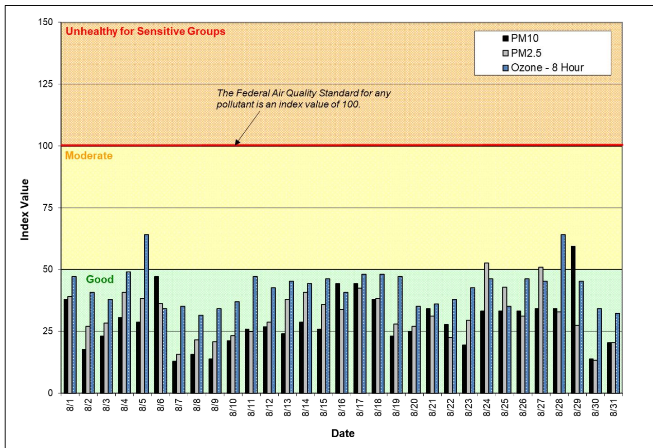
Figure 1: Air Quality Index (AQI) values for August 2020. The data represent the maximum AQI values across all monitoring stations within Spokane County.
