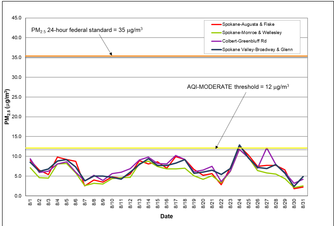
Figure 2: Multi-station 24-hour average PM 2.5 for August 2020; Spokane County.
