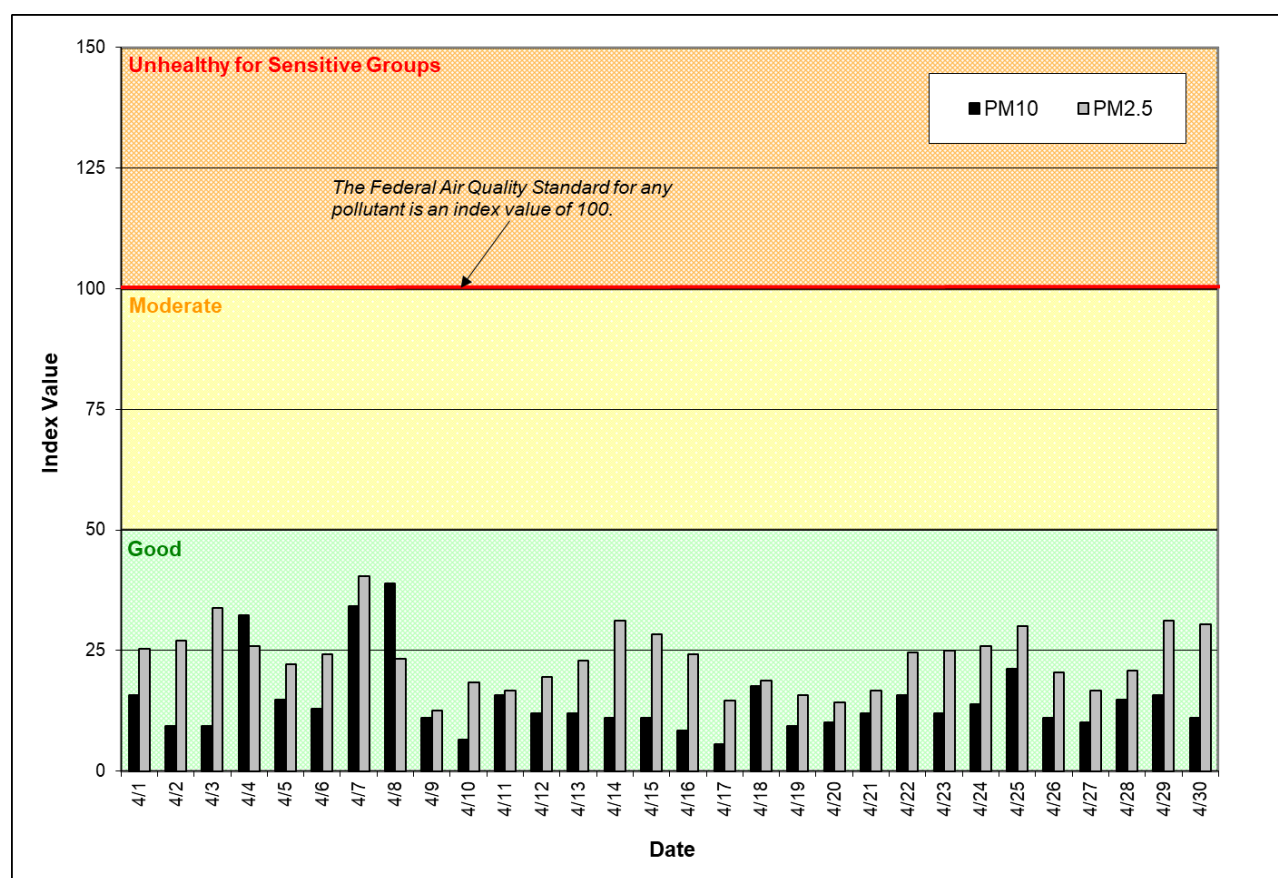
Figure 1: Air Quality Index (AQI) values for April 2022. The data represent the maximum AQI values across all monitoring stations within Spokane County.
