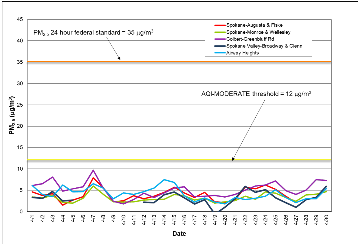
Figure 2: Multi-station 24-hour average PM 2.5 for April 2022; Spokane County.
