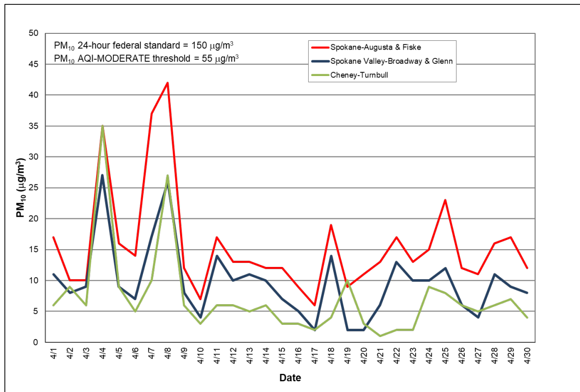
Figure 3: Multi-station 24-hour average PM 10 for April 2022; Spokane County.
