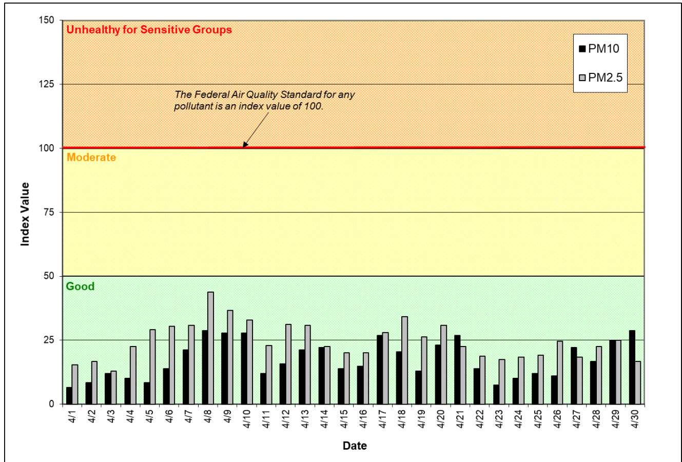
Figure 1: Air Quality Index (AQI) values for April 2020. The data represent the maximum AQI values across all monitoring stations within Spokane County.
