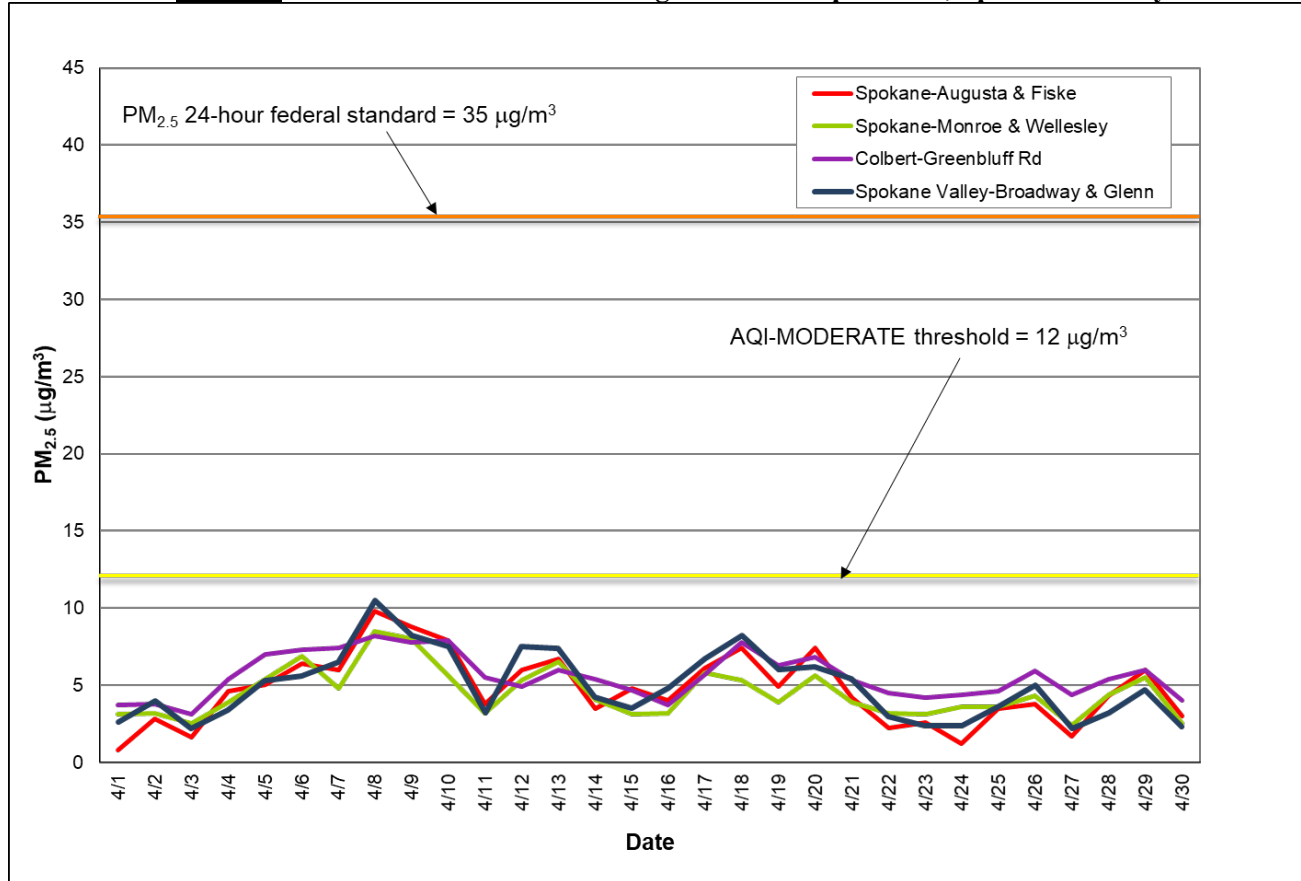
Figure 2: Multi-station 24-hour average PM 2.5 for April 2020; Spokane County.
