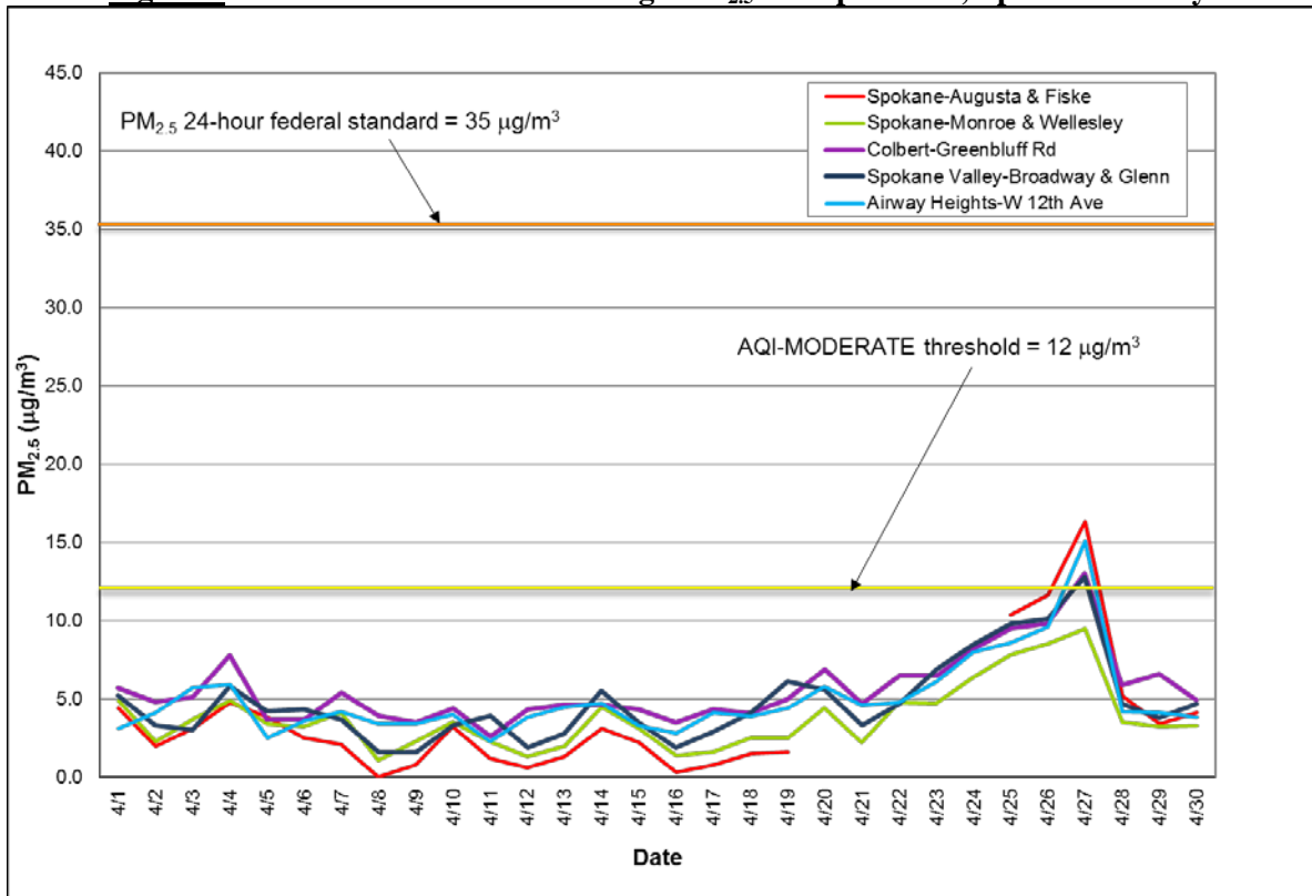
Figure 2: Multi-station 24-hour average PM 2.5 for April 2018; Spokane County.
