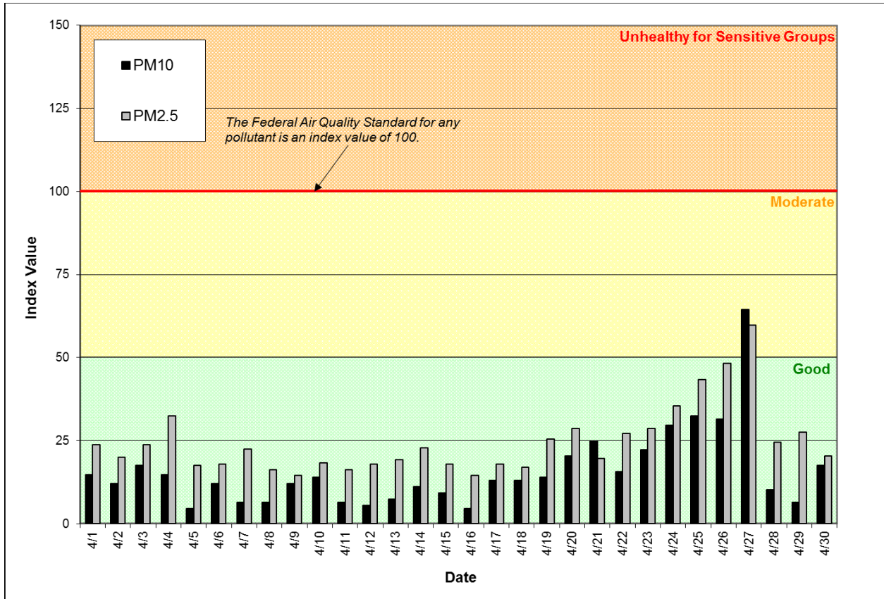
Figure 1: Air Quality Index (AQI) values for April 2018. The data represent the maximum AQI values across all monitoring stations within Spokane County.
