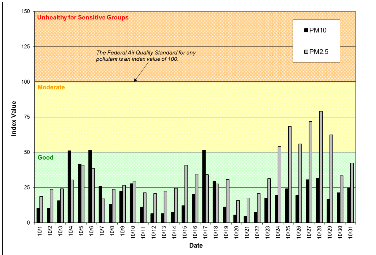
Figure 1: Air Quality Index (AQI) values for October 2017. The data represent the maximum AQI values across all monitoring stations within Spokane County.
