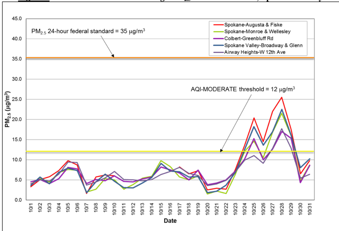
Figure 2: Multi-station 24-hour average PM 2.5 for October 2017; Spokane County.
