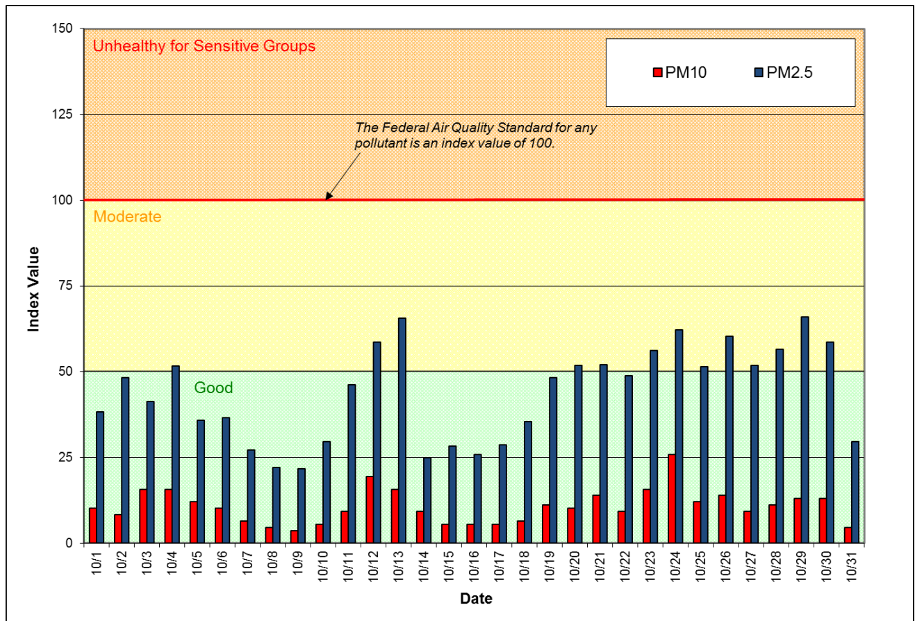
Figure 1: Air Quality Index (AQI) values for October 2016. The data represent the maximum AQI values across all monitoring stations within Spokane County.
