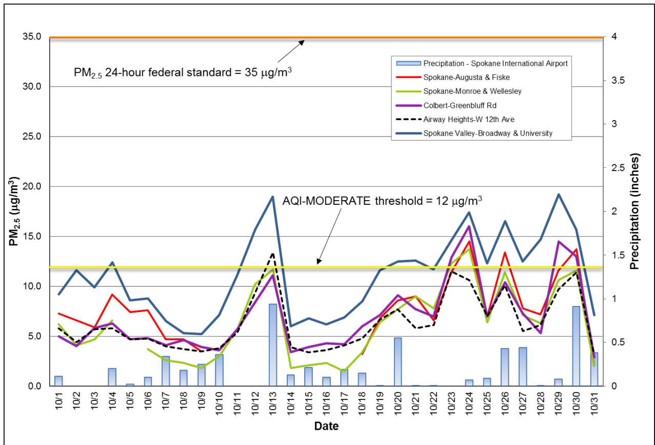
Figure 2: Multi-station 24-hour average PM 2.5 and precipitation for October 2016; Spokane County.
