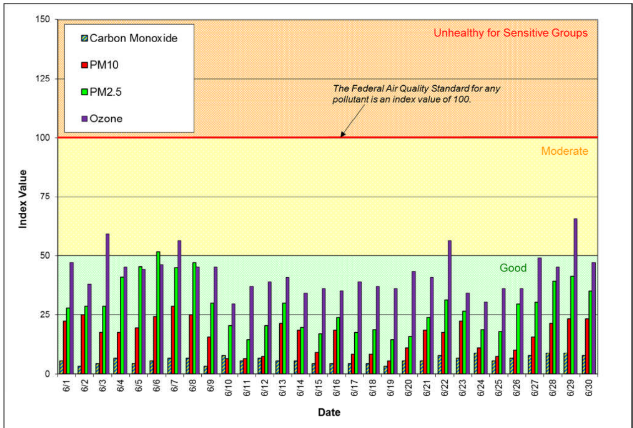
Figure 1: Air Quality Index (AQI) values for June 2016. The data represent the maximum AQI values across all monitoring stations within Spokane County.
