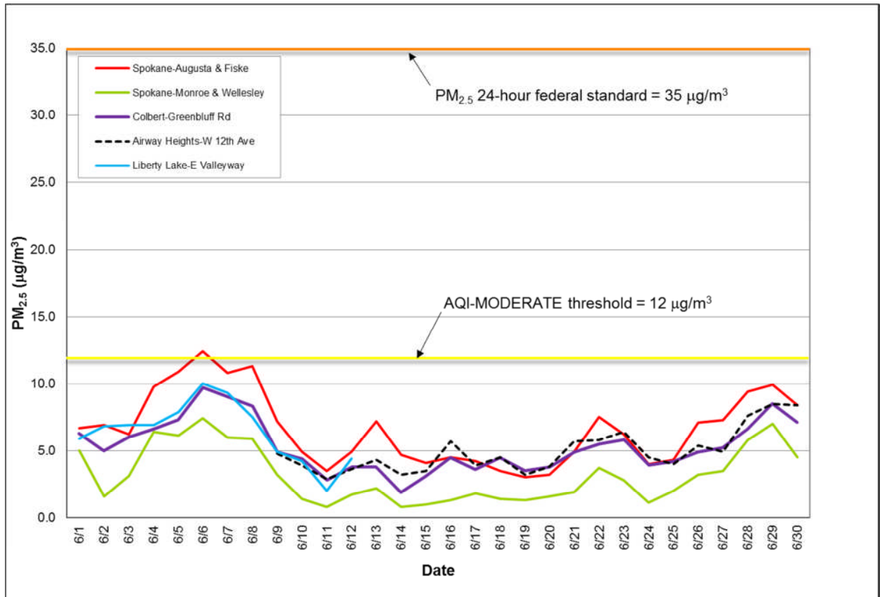
Figure 2: Multi-station 24-hour average PM 2.5 for June 2016; Spokane County.
