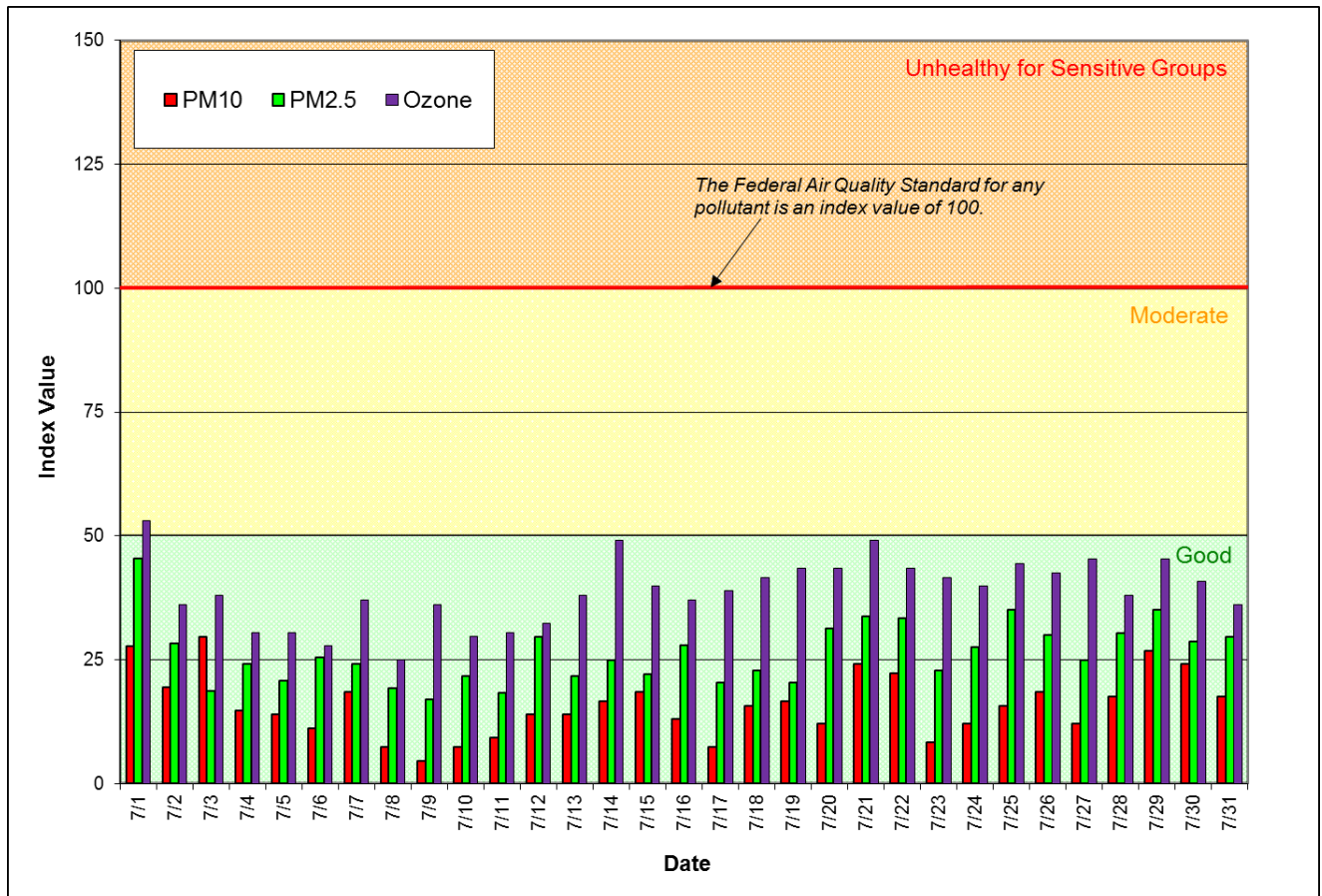
Figure 1: Air Quality Index (AQI) values for July 2016. The data represent the maximum AQI values across all monitoring stations within Spokane County.
