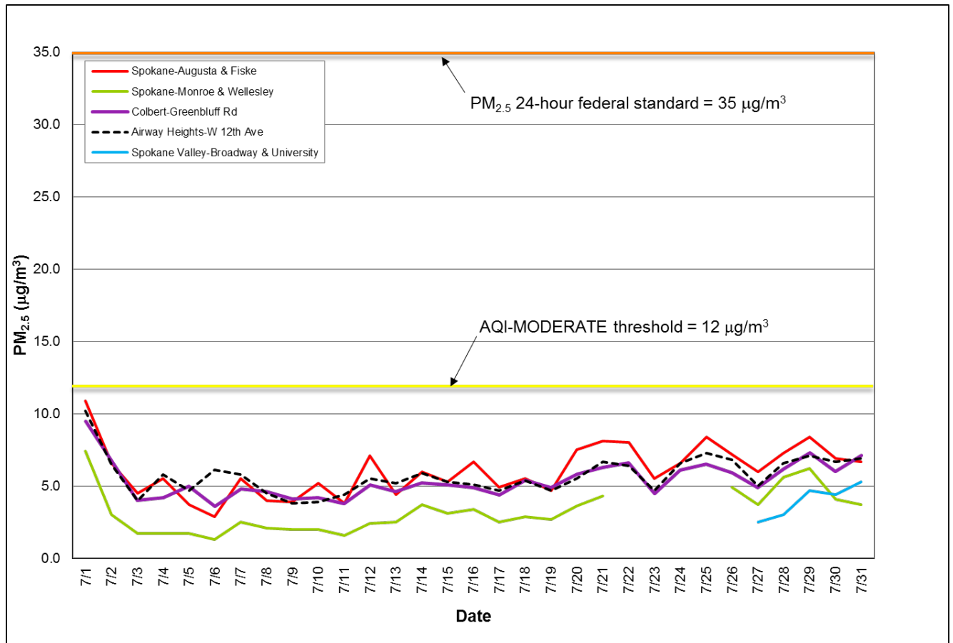
Figure 2: Multi-station 24-hour average PM 2.5 for July 2016; Spokane County.
